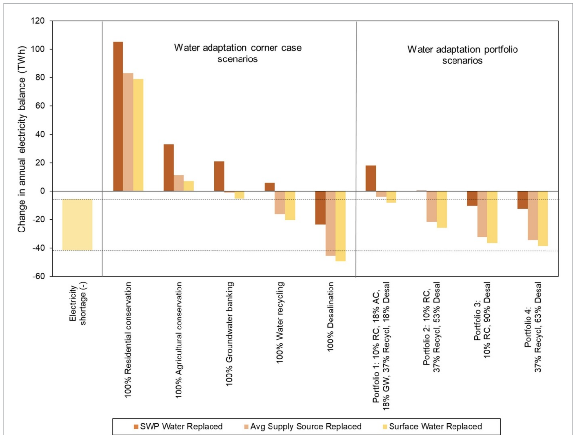
Figure 3. Energy impacts of water adaptations compared to direct climate impacts on California electricity balance. Dotted lines indicate the range of the annual electricity shortage from direct climate change impacts by the end-century in California (from figure 2(b)). The panels on the right show the annual energy consumption or savings impacts of water adaptations to meet the worst-case end-century water shortage in California. Corner cases meet the full water shortage with a single adaptation; portfolios include combinations of measures, as indicated by the percentage share. RC = Residential conservation; AC = Agricultural conservation; GW = Groundwater banking; Recycl = Water recycling for potable reuse; Desal = Desalination. Colors indicate water sources replaced by adaptations. SWP = State Water Project. Positive indicates surplus, negative indicates shortage.
